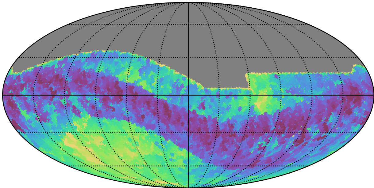
too_elab_r8_d3_gz_v3.4_10yrs All sky i band: Min skyBrightness
