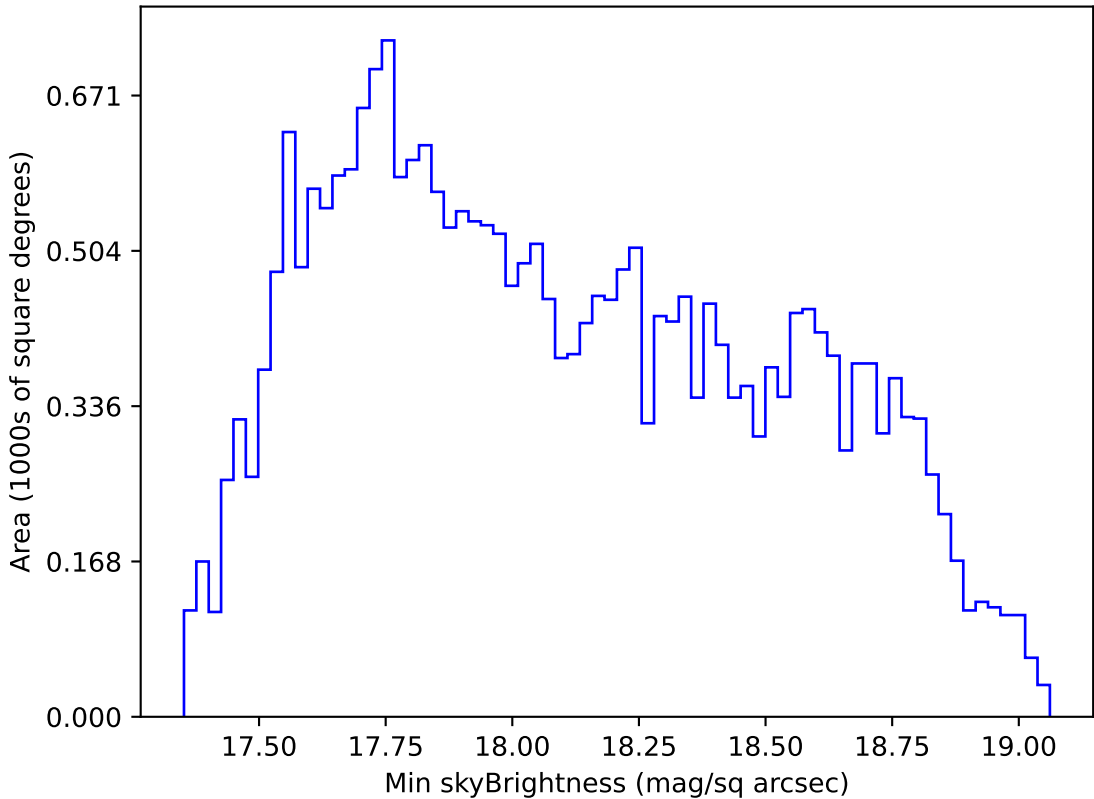
too_elab_r8_d3_gz_v3.4_10yrs All sky i band: Min skyBrightness
