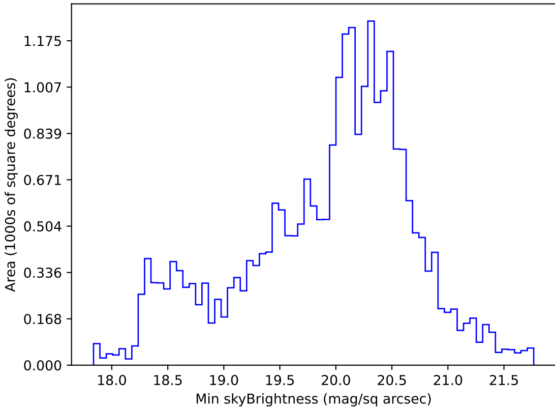
too_elab_r8_d3_gz_v3.4_10yrs All sky g band: Min skyBrightness
