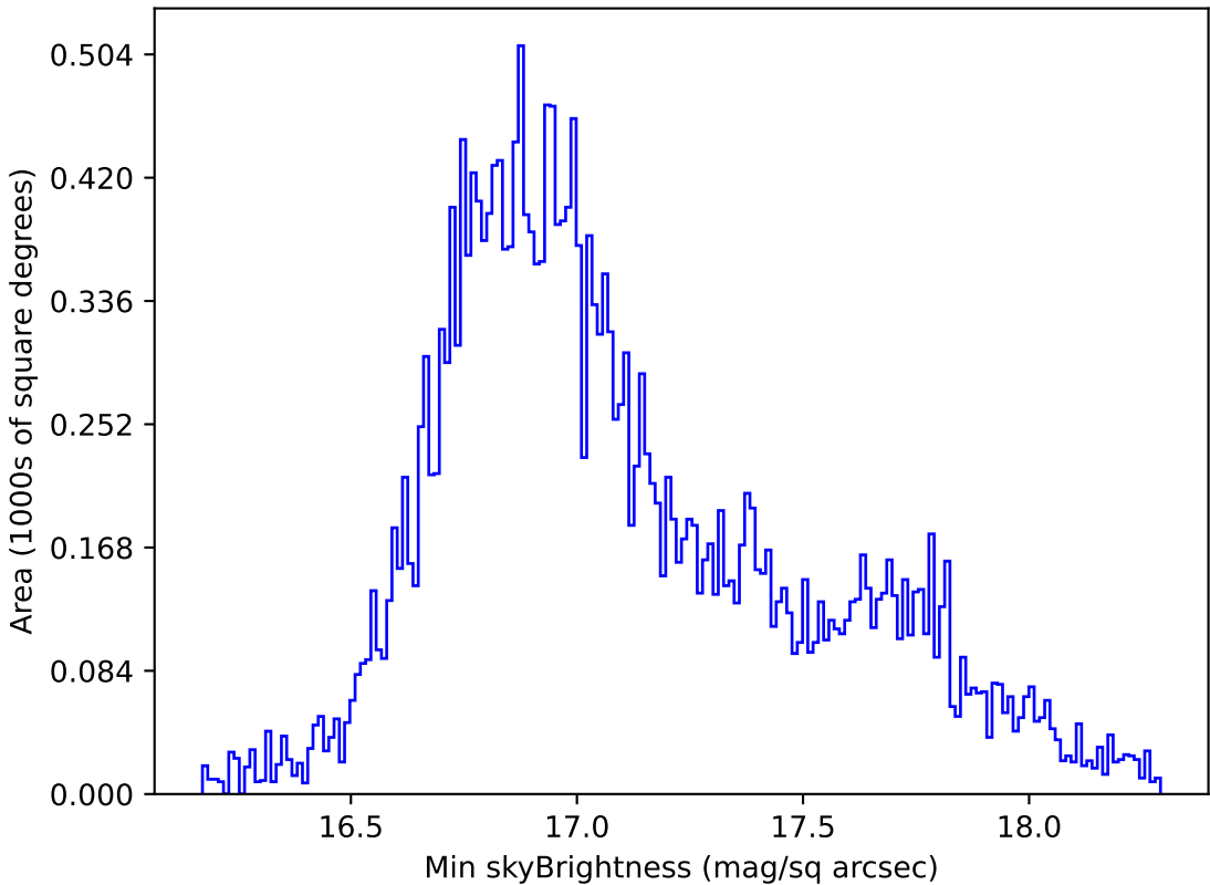
too_elab_r8_d3_gz_v3.4_10yrs All sky all bands: Min skyBrightness
