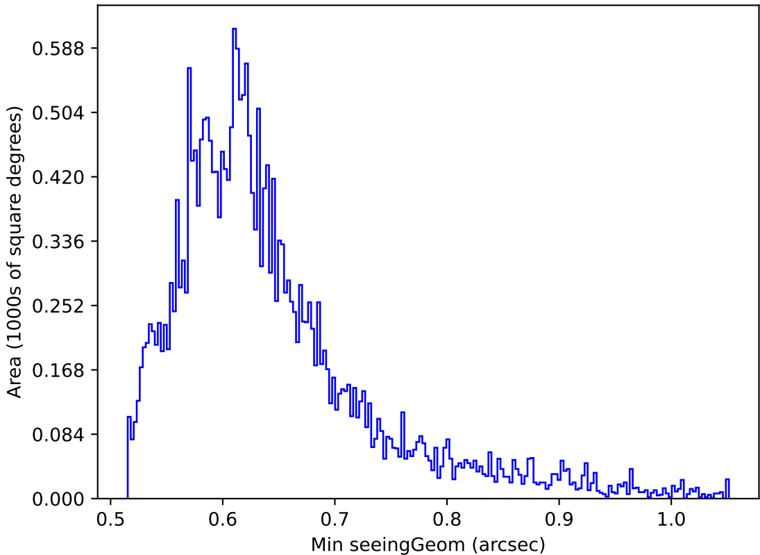
too_elab_r8_d3_gz_v3.4_10yrs Yr 1 z band: Min seeingGeom
