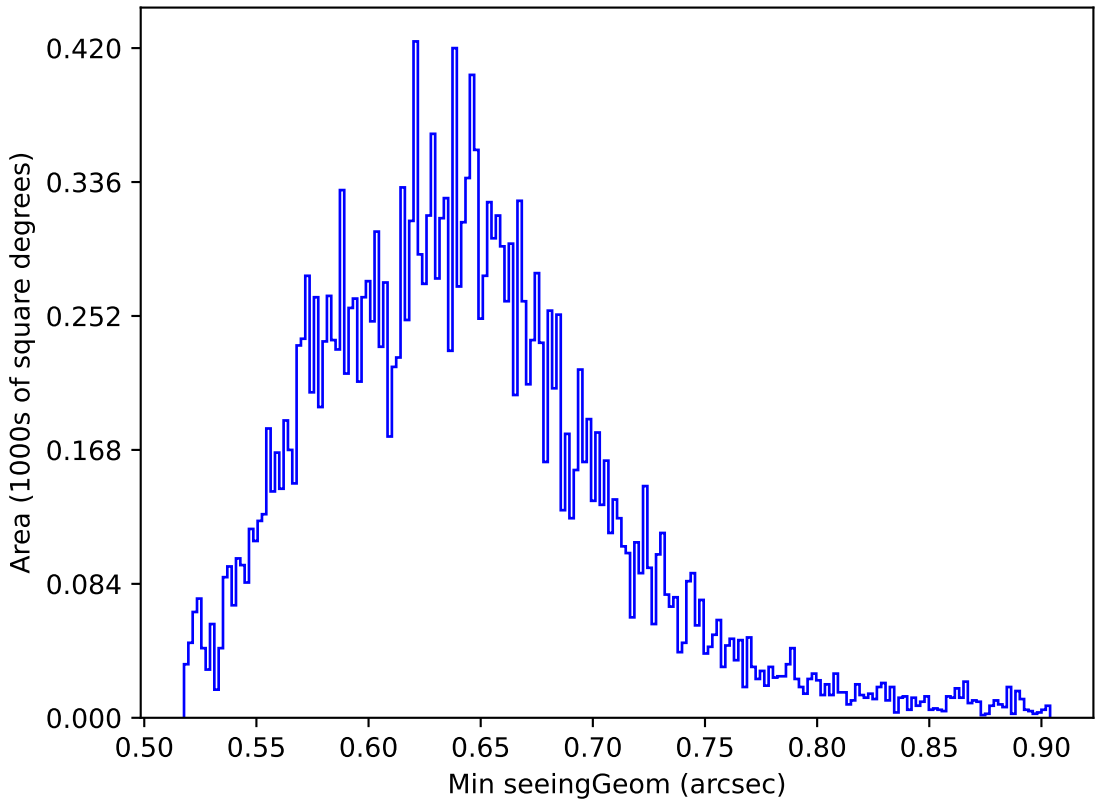
too_elab_r8_d3_gz_v3.4_10yrs Yr 1 y band: Min seeingGeom
