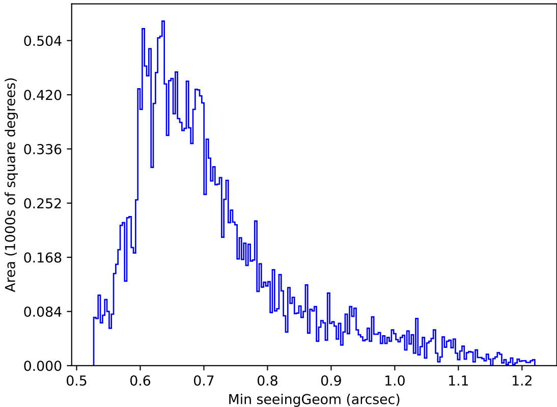
too_elab_r8_d3_gz_v3.4_10yrs Yr 1 g band: Min seeingGeom
