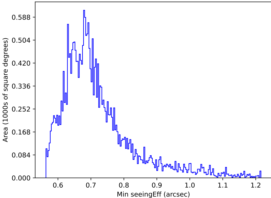
too_elab_r8_d3_gz_v3.4_10yrs Yr 1 z band: Min seeingEff
