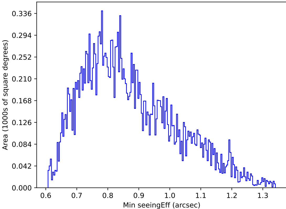
too_elab_r8_d3_gz_v3.4_10yrs Yr 1 u band: Min seeingEff
