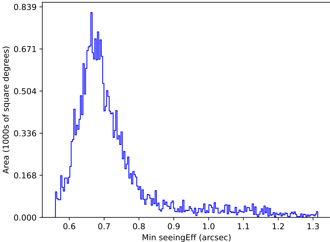
too_elab_r8_d3_gz_v3.4_10yrs Yr 1 r band: Min seeingEff
