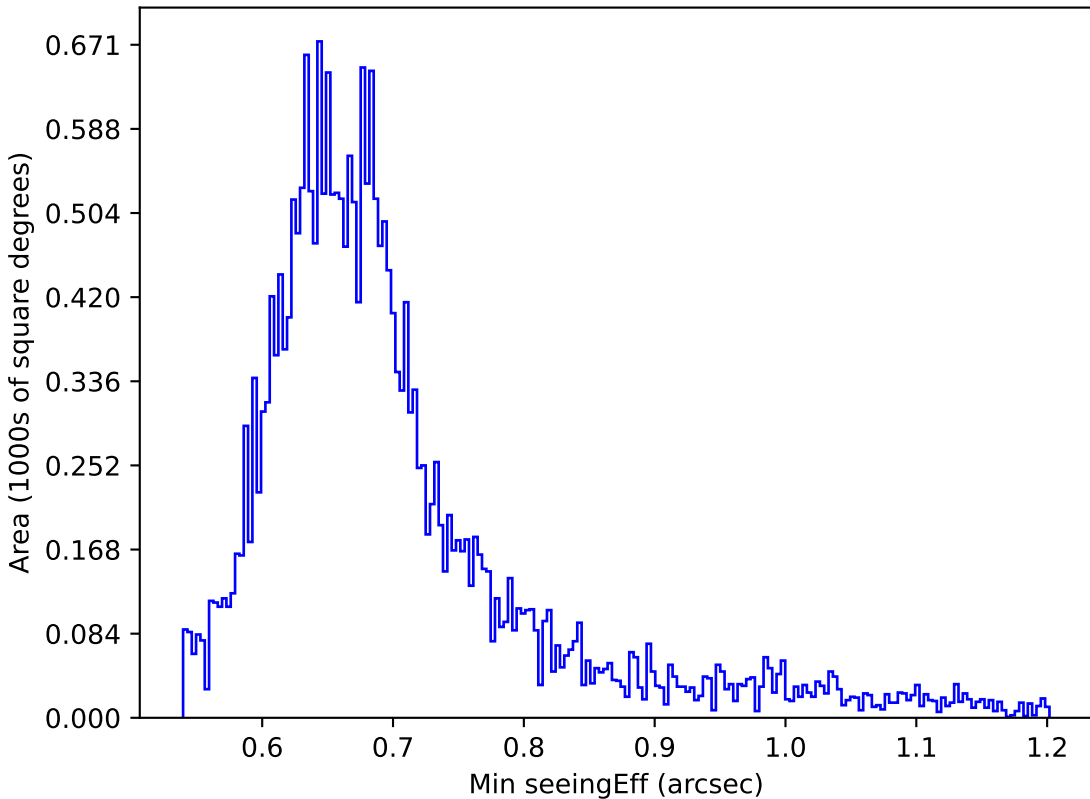
too_elab_r8_d3_gz_v3.4_10yrs Yr 1 i band: Min seeingEff
