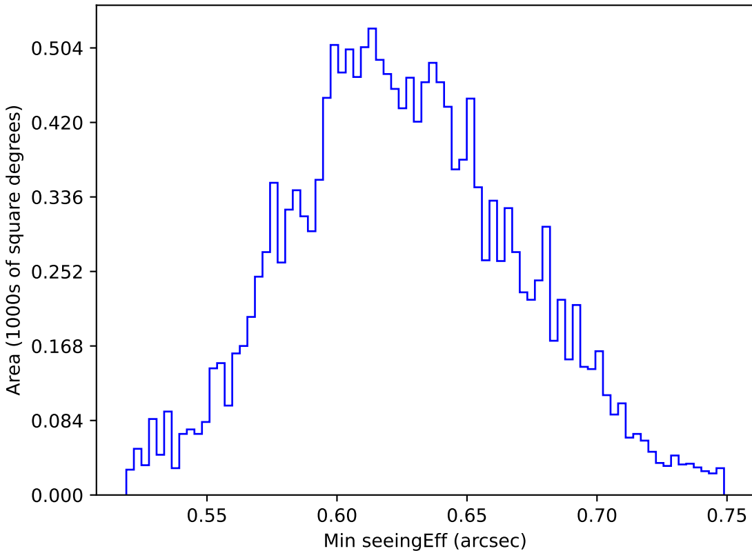
too_elab_r8_d3_gz_v3.4_10yrs WFD y band: Min seeingEff
