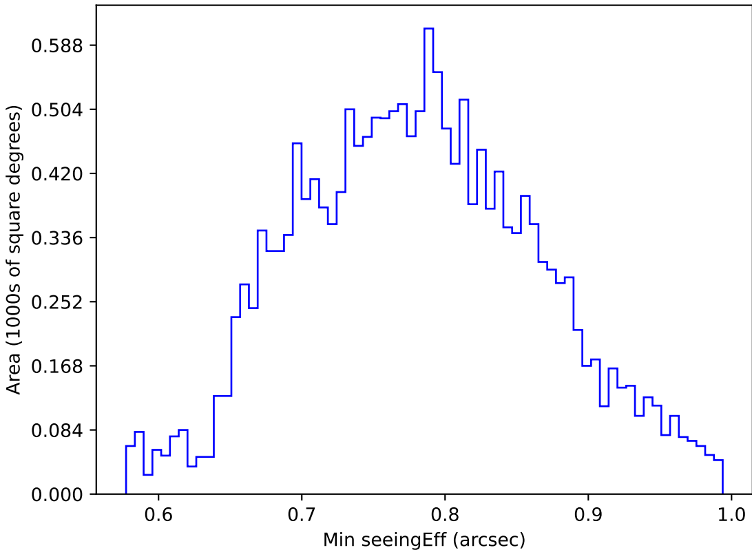
too_elab_r8_d3_gz_v3.4_10yrs WFD u band: Min seeingEff
