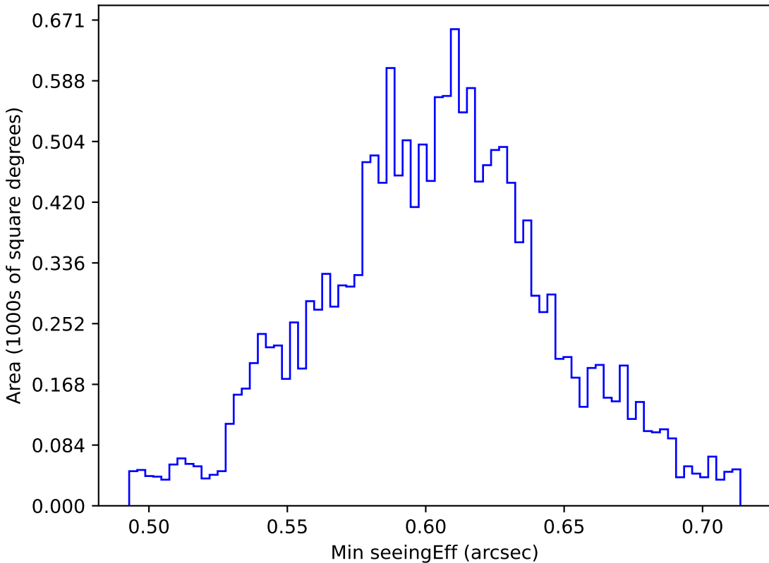
too_elab_r8_d3_gz_v3.4_10yrs WFD i band: Min seeingEff
