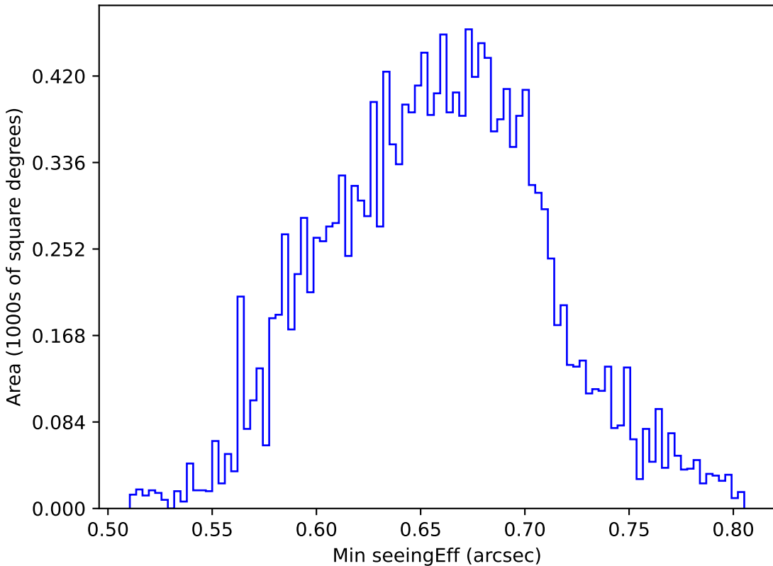
too_elab_r8_d3_gz_v3.4_10yrs WFD g band: Min seeingEff
