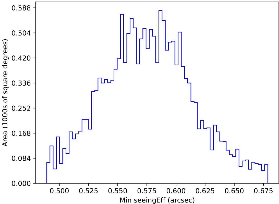
too_elab_r8_d3_gz_v3.4_10yrs WFD all bands: Min seeingEff
