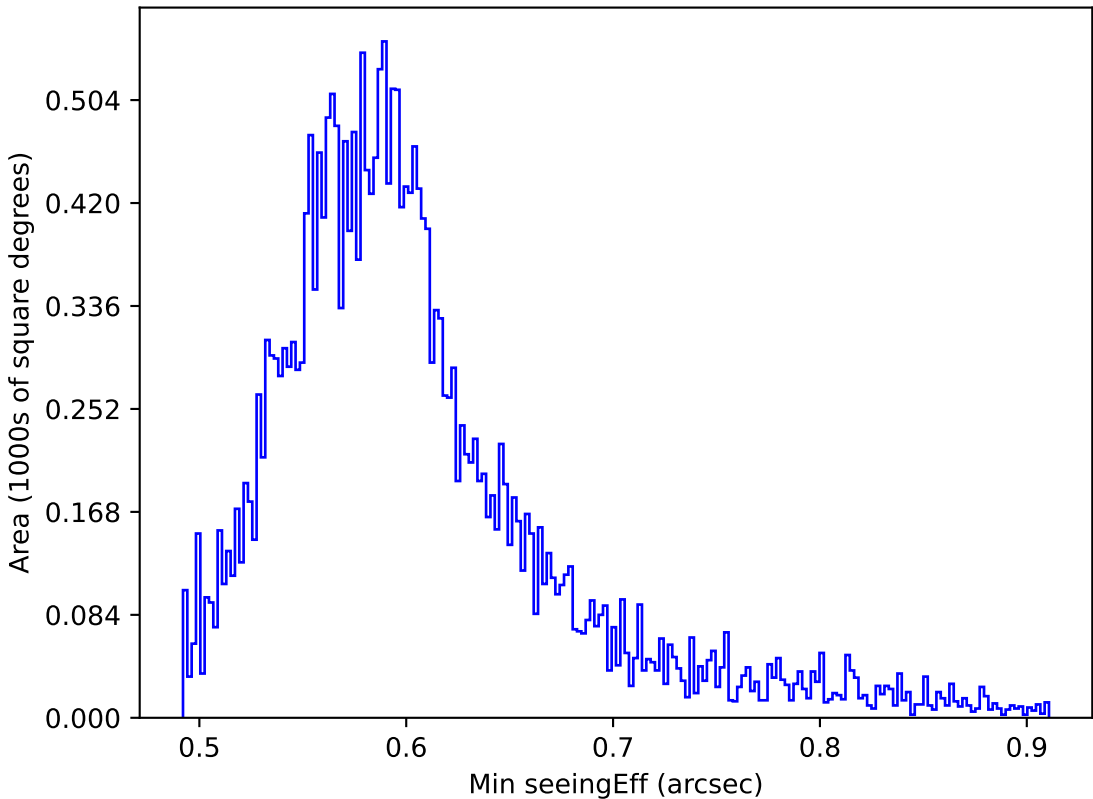
too_elab_r8_d3_gz_v3.4_10yrs All sky all bands: Min seeingEff
