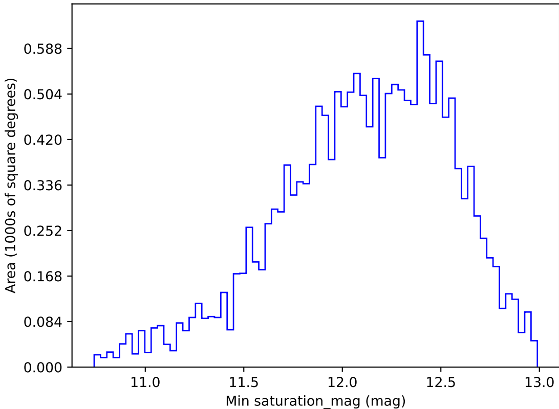
too_elab_r8_d3_gz_v3.4_10yrs WFD z band: Min saturation_mag
