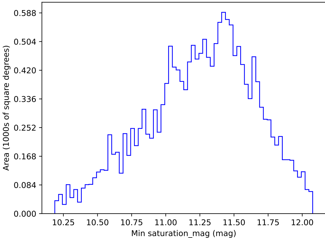
too_elab_r8_d3_gz_v3.4_10yrs WFD y band: Min saturation_mag
