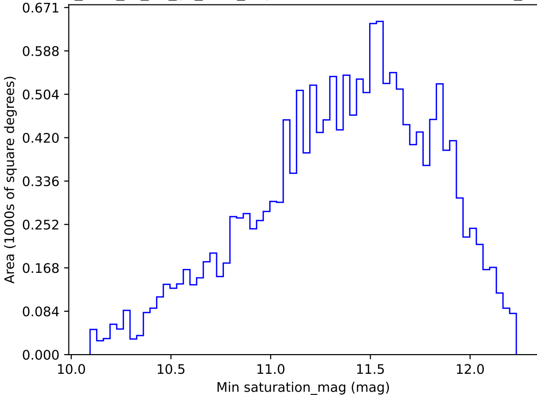
too_elab_r8_d3_gz_v3.4_10yrs WFD u band: Min saturation_mag
