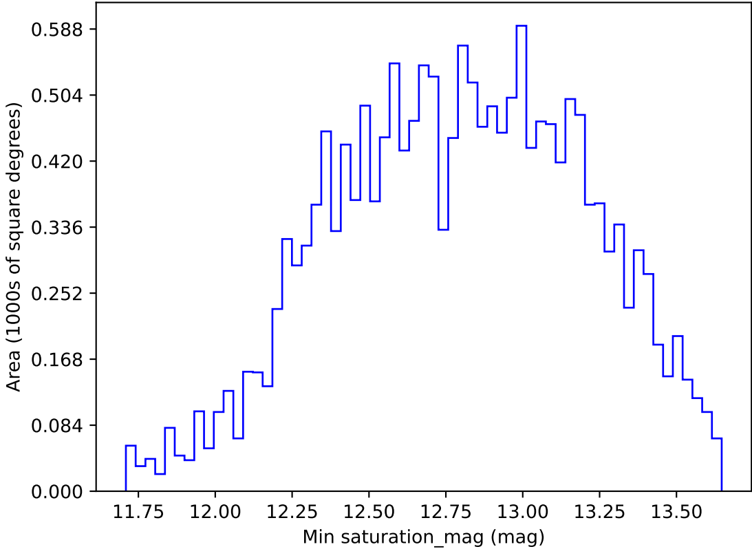
too_elab_r8_d3_gz_v3.4_10yrs WFD g band: Min saturation_mag
