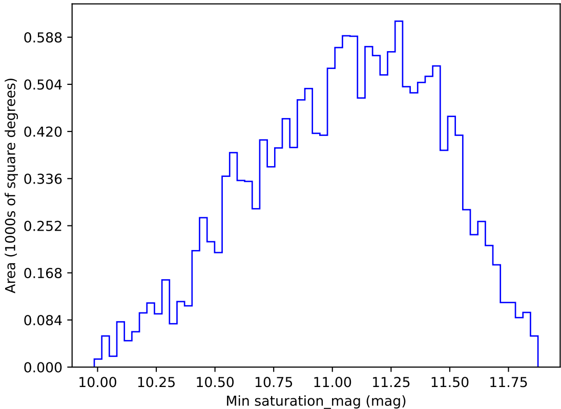
too_elab_r8_d3_gz_v3.4_10yrs WFD all bands: Min saturation_mag
