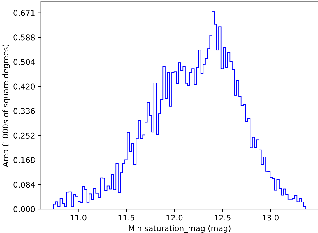
too_elab_r8_d3_gz_v3.4_10yrs All sky z band: Min saturation_mag
