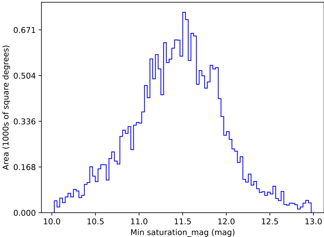
too_elab_r8_d3_gz_v3.4_10yrs All sky u band: Min saturation_mag
