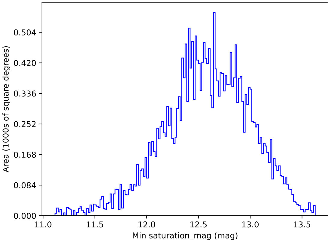
too_elab_r8_d3_gz_v3.4_10yrs All sky r band: Min saturation_mag
