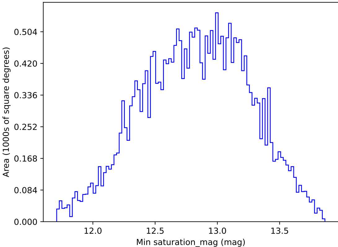
too_elab_r8_d3_gz_v3.4_10yrs All sky g band: Min saturation_mag
