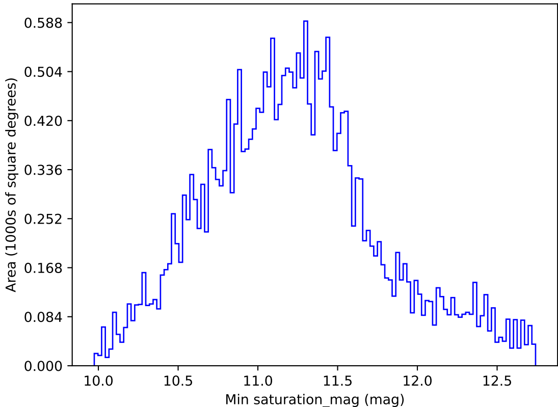
too_elab_r8_d3_gz_v3.4_10yrs All sky all bands: Min saturation_mag
