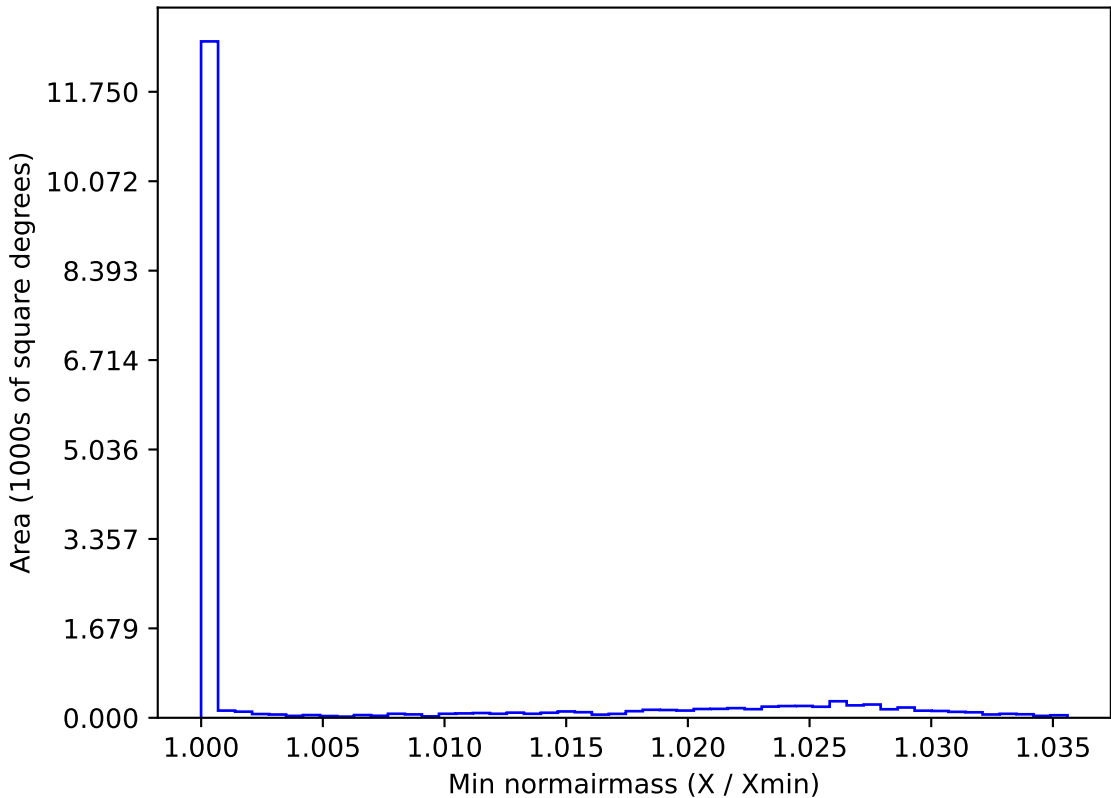
too_elab_r8_d3_gz_v3.4_10yrs WFD z band: Min normairmass
