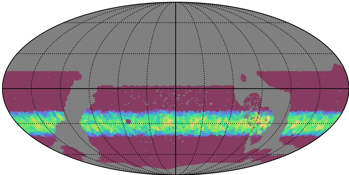
too_elab_r8_d3_gz_v3.4_10yrs WFD y band: Min normairmass
