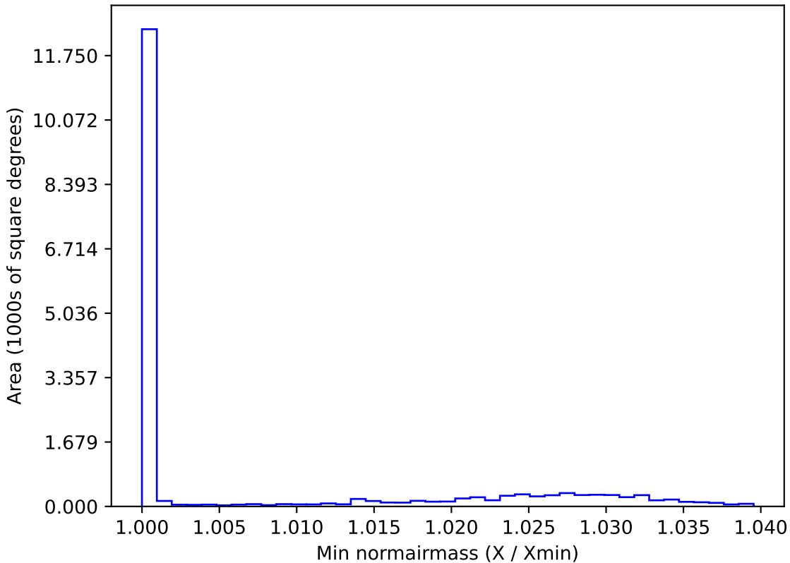
too_elab_r8_d3_gz_v3.4_10yrs WFD y band: Min normairmass
