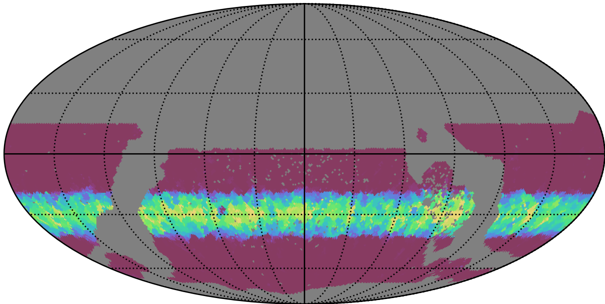
too_elab_r8_d3_gz_v3.4_10yrs WFD u band: Min normairmass
