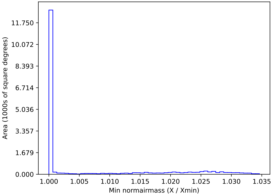
too_elab_r8_d3_gz_v3.4_10yrs WFD r band: Min normairmass
