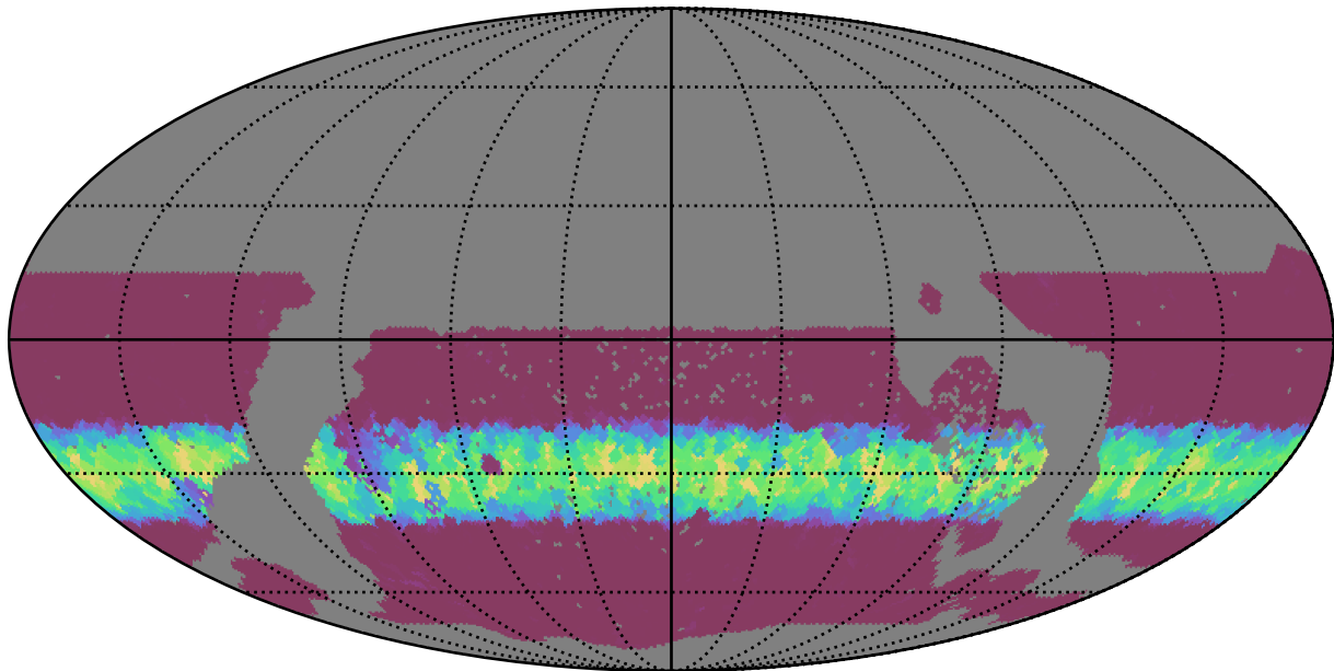
too_elab_r8_d3_gz_v3.4_10yrs WFD g band: Min normairmass
