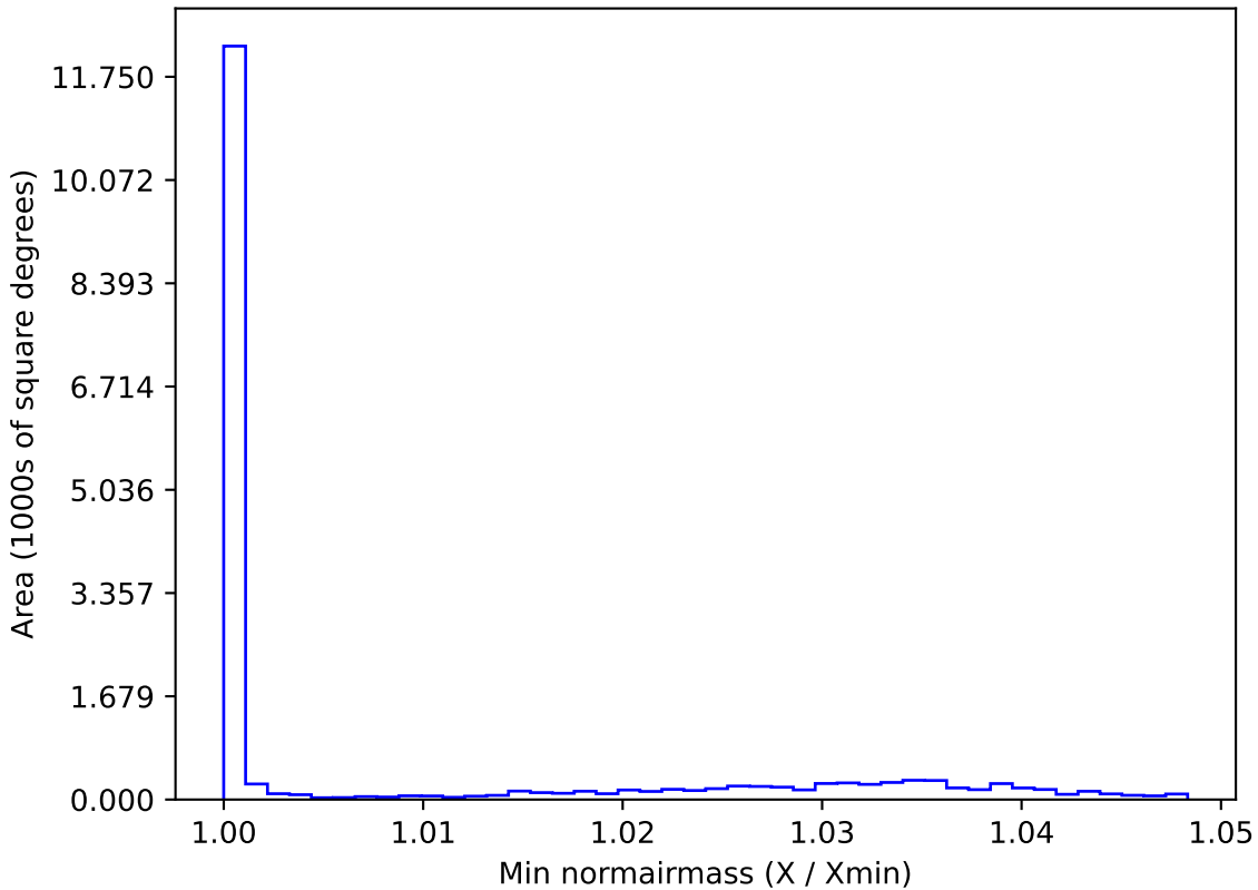
too_elab_r8_d3_gz_v3.4_10yrs WFD g band: Min normairmass
