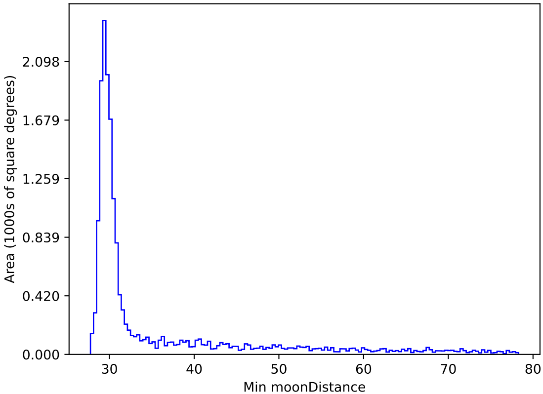
too_elab_r8_d3_gz_v3.4_10yrs WFD z band: Min moonDistance
