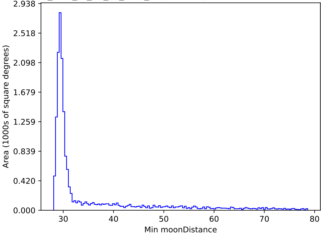
too_elab_r8_d3_gz_v3.4_10yrs WFD y band: Min moonDistance
