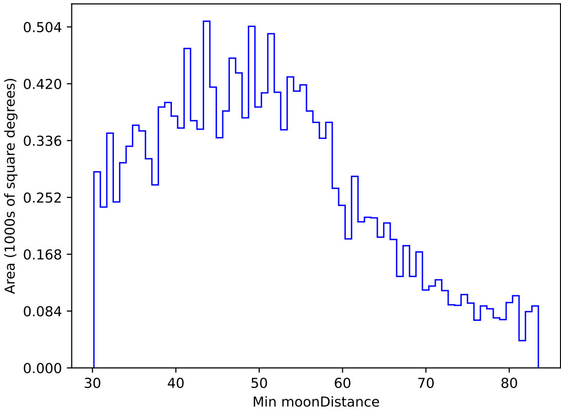
too_elab_r8_d3_gz_v3.4_10yrs WFD u band: Min moonDistance
