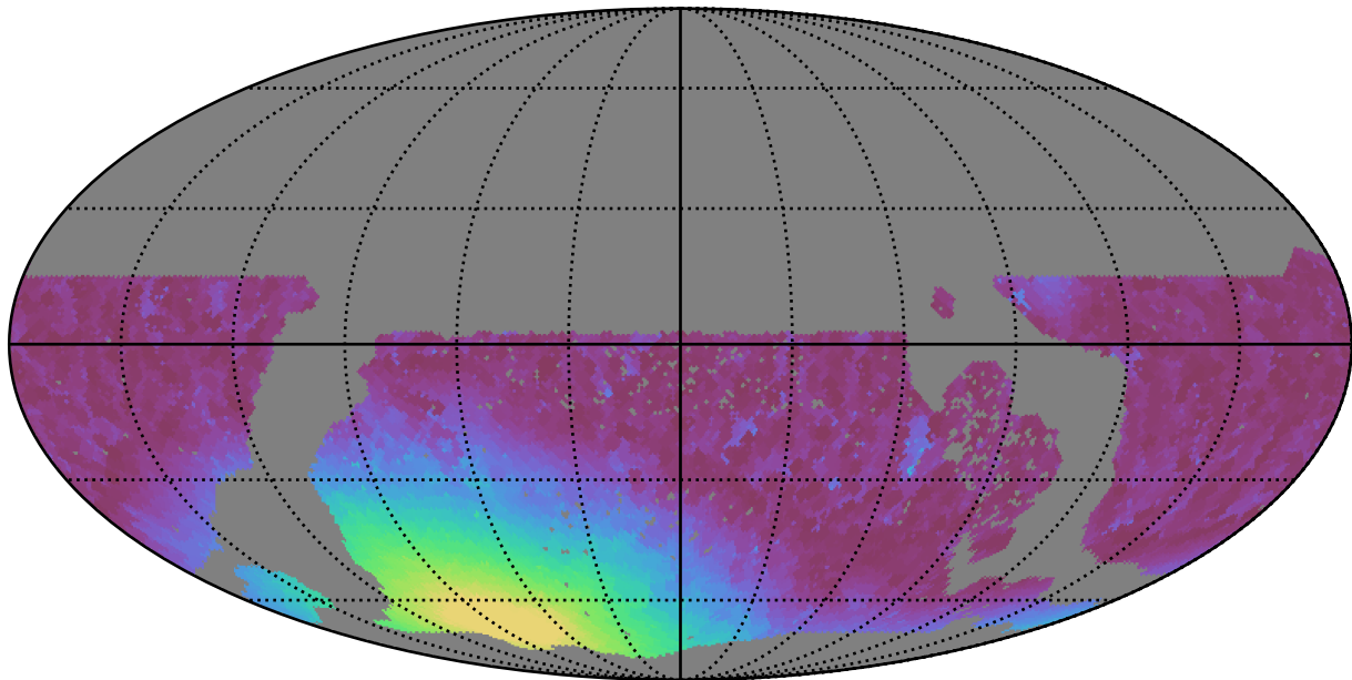
too_elab_r8_d3_gz_v3.4_10yrs WFD r band: Min moonDistance
