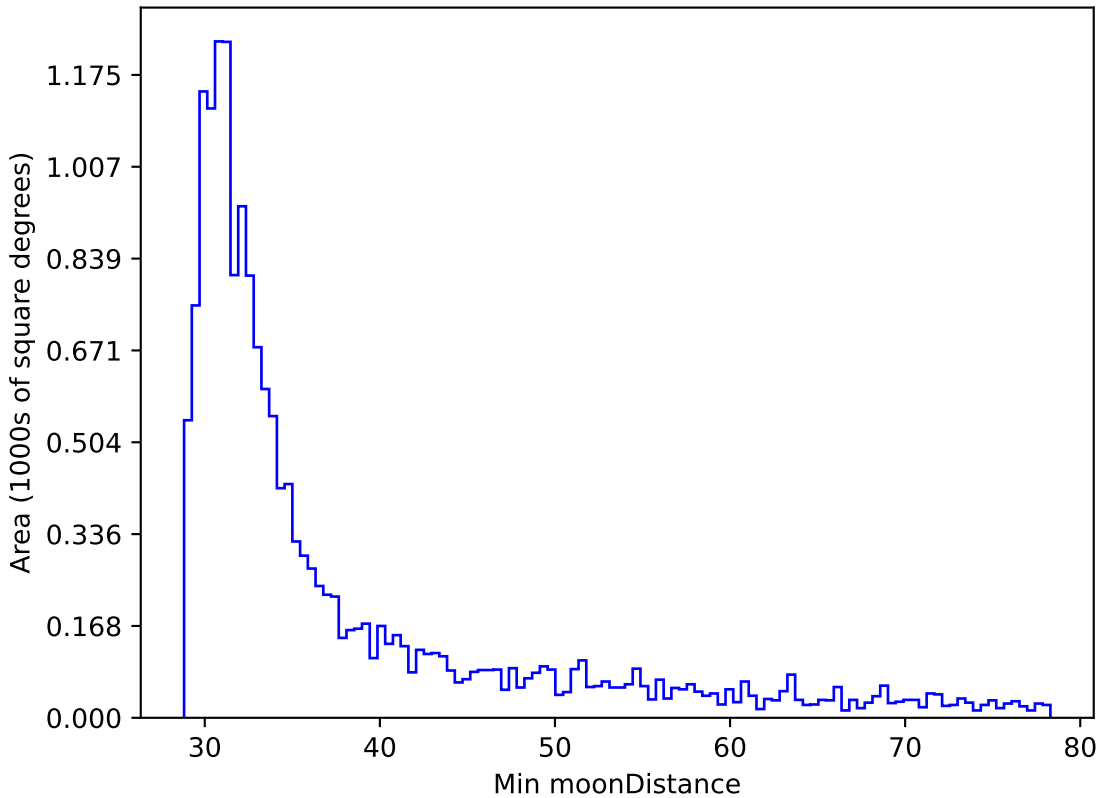
too_elab_r8_d3_gz_v3.4_10yrs WFD r band: Min moonDistance
