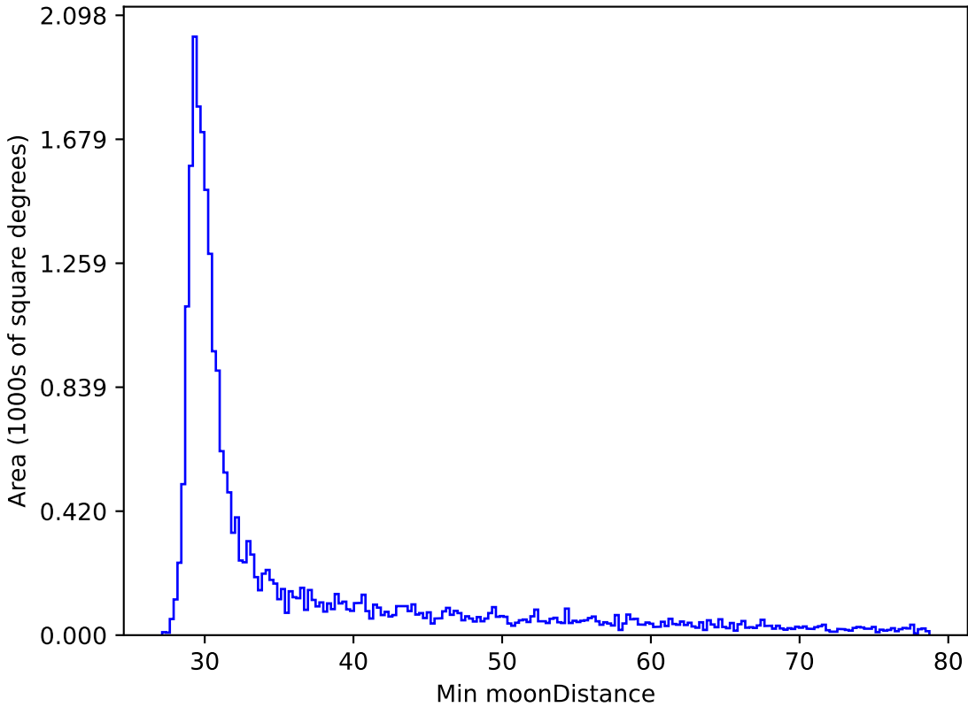
too_elab_r8_d3_gz_v3.4_10yrs All sky z band: Min moonDistance
