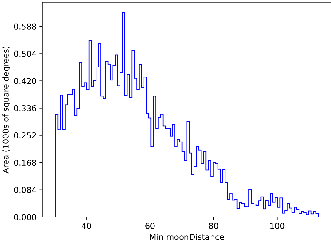
too_elab_r8_d3_gz_v3.4_10yrs All sky u band: Min moonDistance
