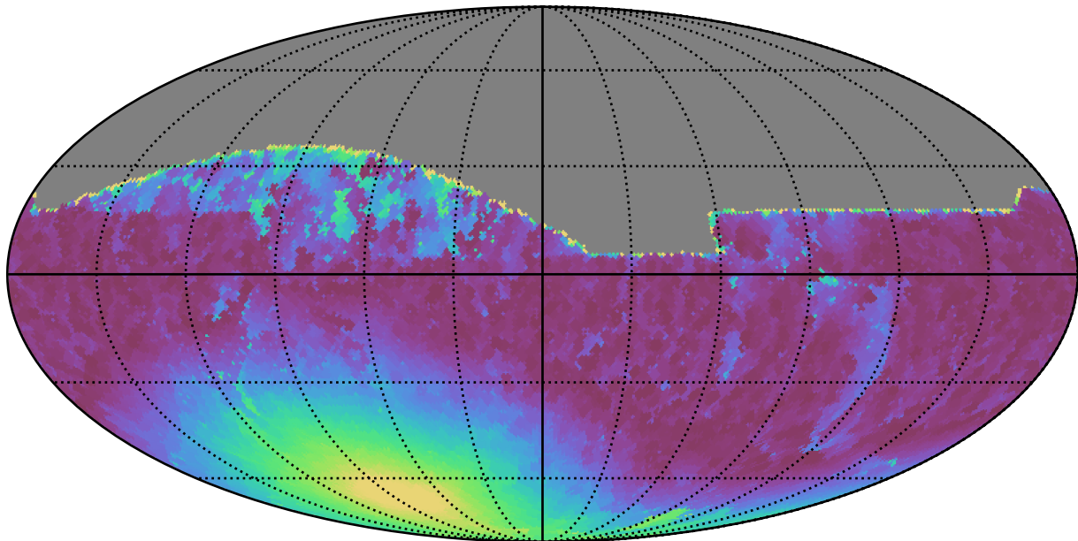
too_elab_r8_d3_gz_v3.4_10yrs All sky r band: Min moonDistance
