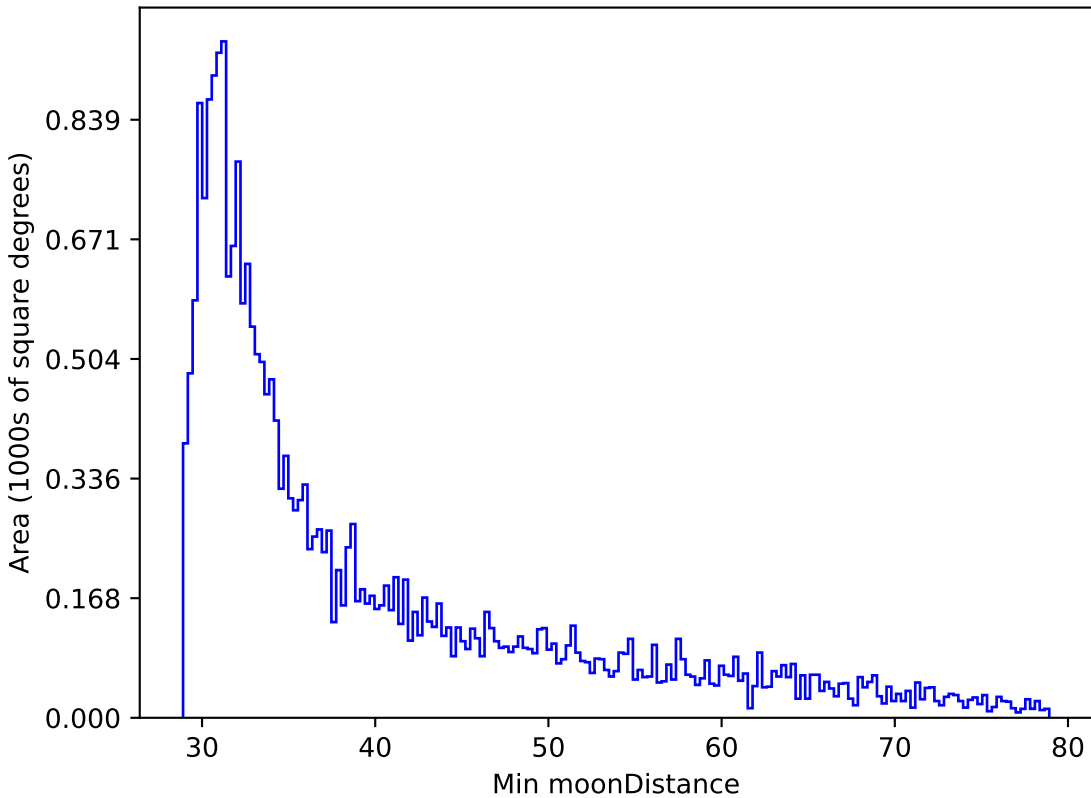
too_elab_r8_d3_gz_v3.4_10yrs All sky r band: Min moonDistance
