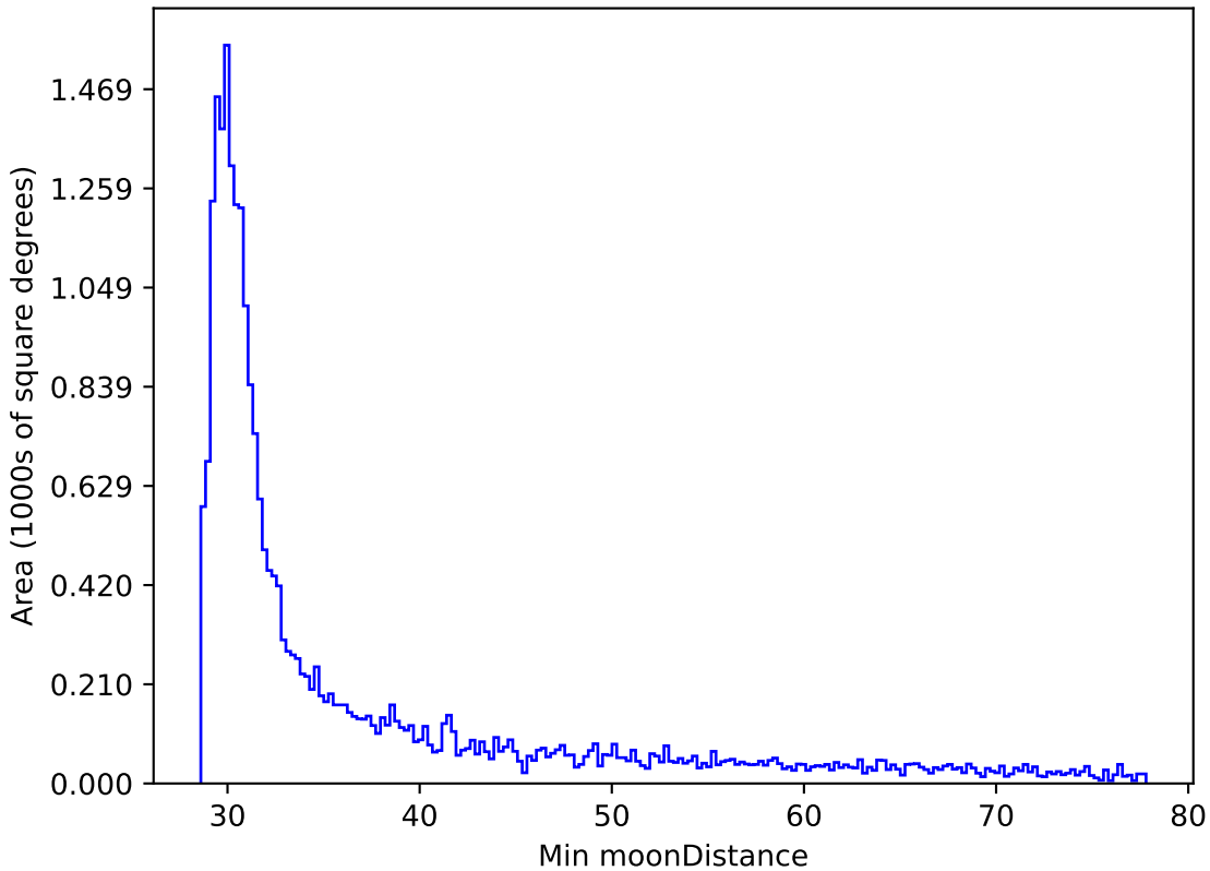
too_elab_r8_d3_gz_v3.4_10yrs All sky i band: Min moonDistance
