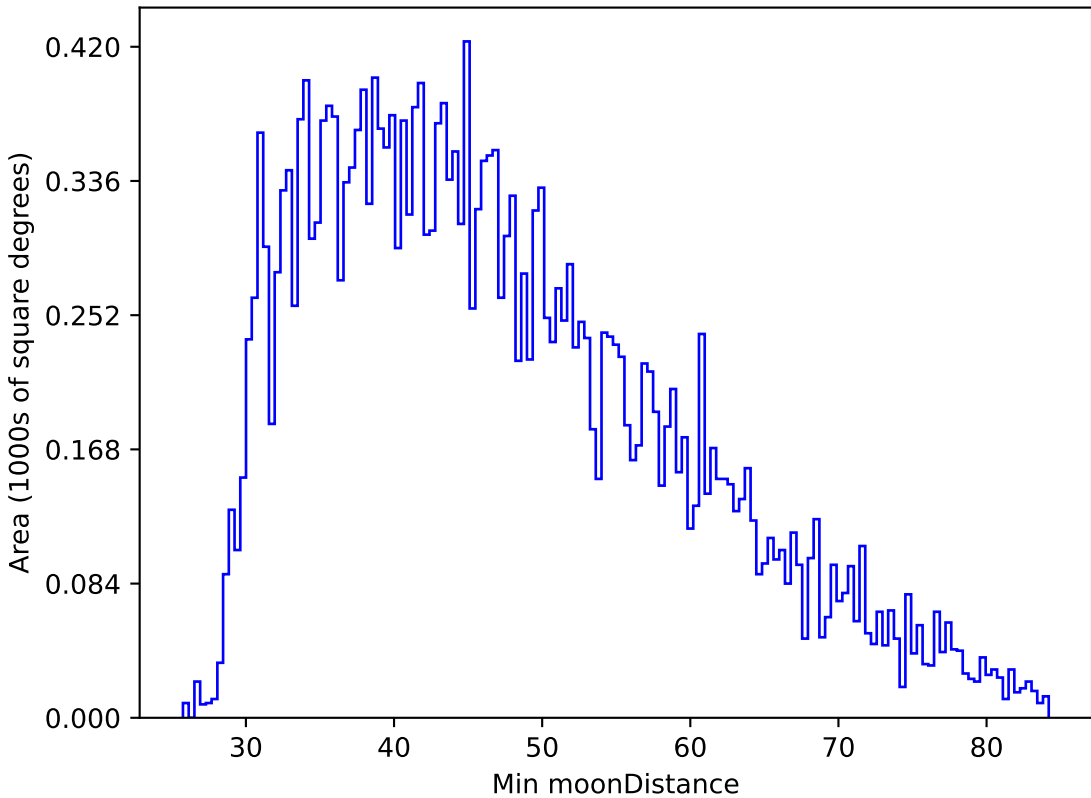
too_elab_r8_d3_gz_v3.4_10yrs All sky g band: Min moonDistance
