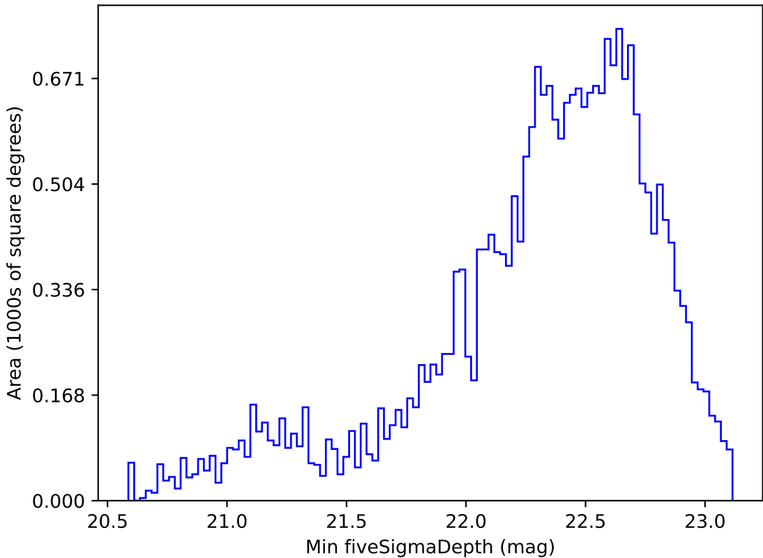
too_elab_r8_d3_gz_v3.4_10yrs Yr 1 z band: Min fiveSigmaDepth
