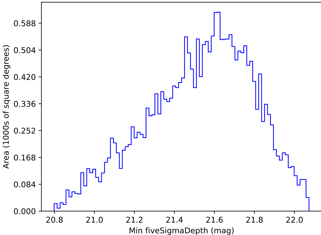
too_elab_r8_d3_gz_v3.4_10yrs Yr 1 y band: Min fiveSigmaDepth
