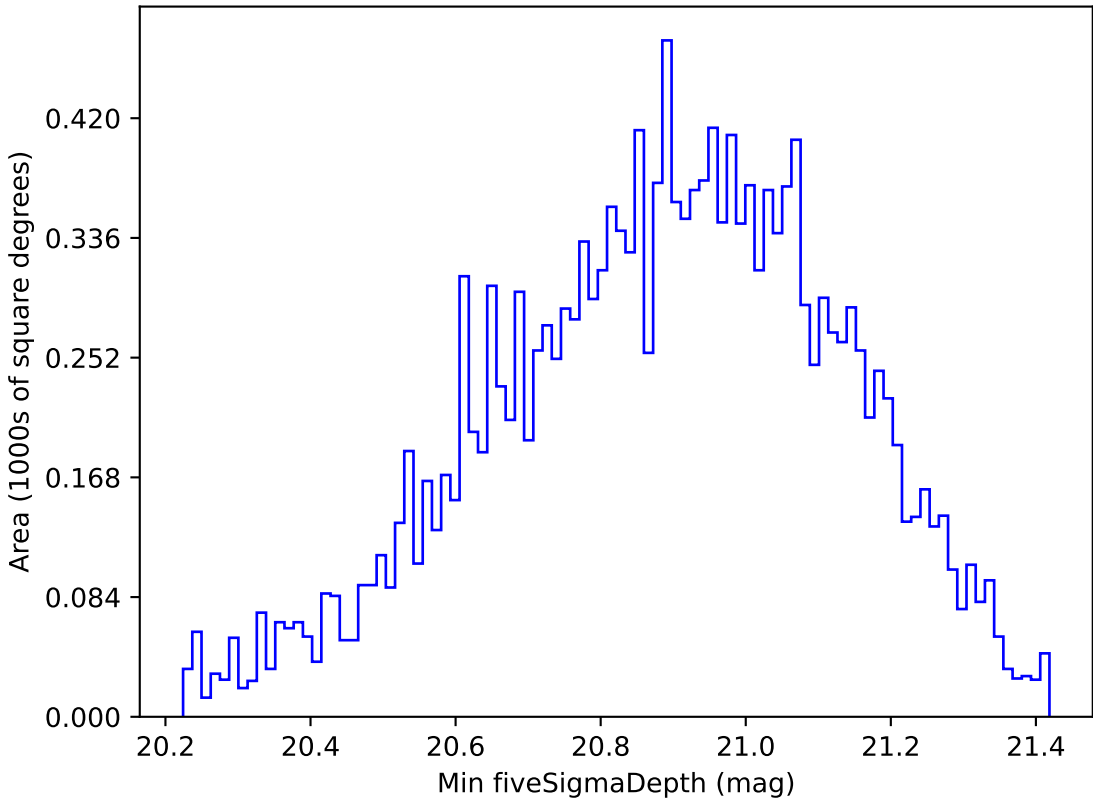
too_elab_r8_d3_gz_v3.4_10yrs WFD y band: Min fiveSigmaDepth
