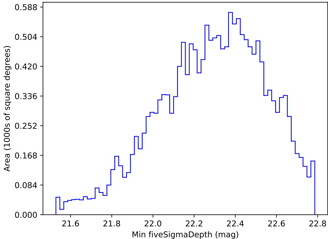
too_elab_r8_d3_gz_v3.4_10yrs WFD u band: Min fiveSigmaDepth
