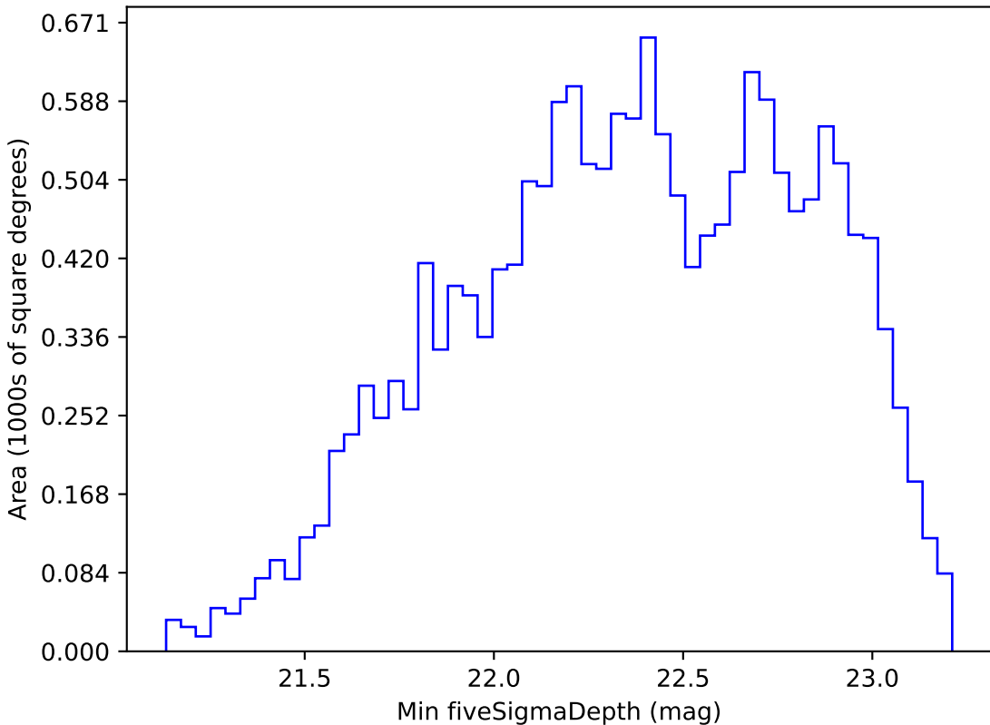
too_elab_r8_d3_gz_v3.4_10yrs WFD r band: Min fiveSigmaDepth
